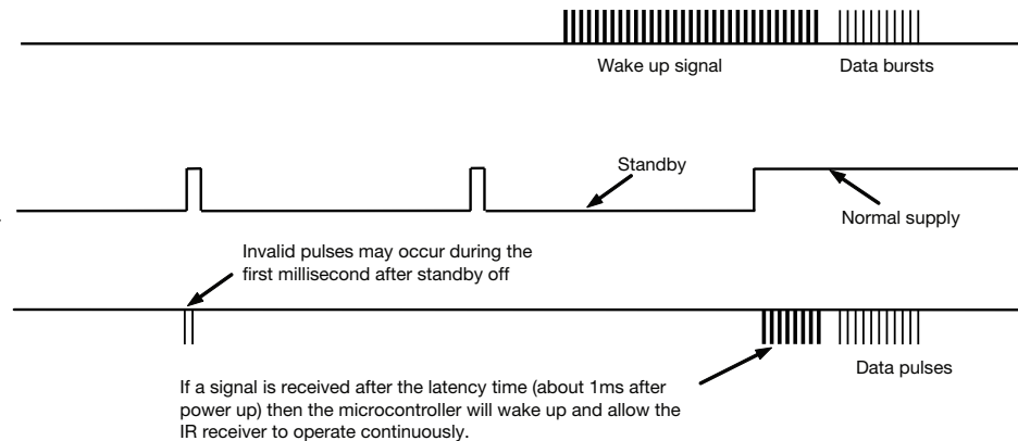
Fig. 6 - Example for a Battery-Saving Mode with TSOP3xxxx IR Receivers
